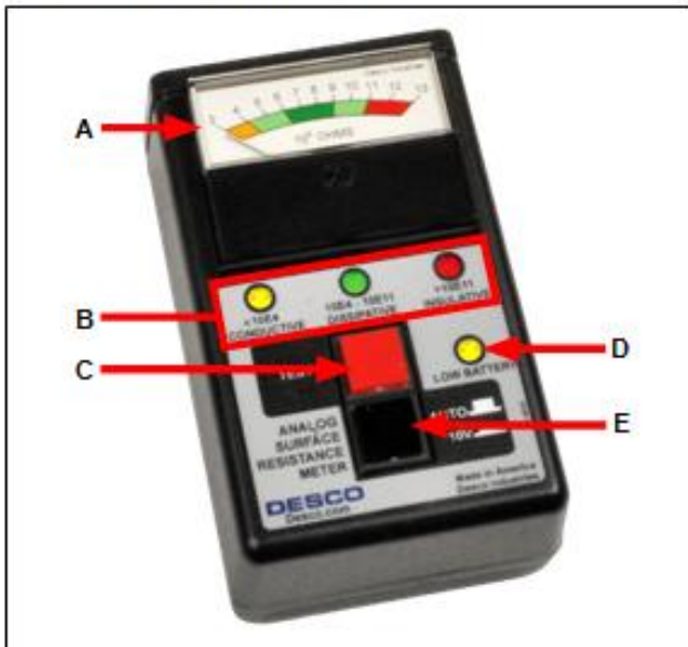
Figure 2. Analog Surface Resistance Meter features and components
